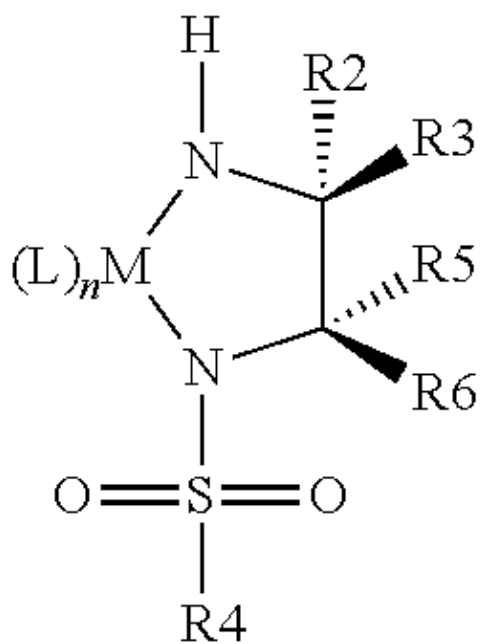
amido-sulfonamidate (shown by ruthenium compound 1)
