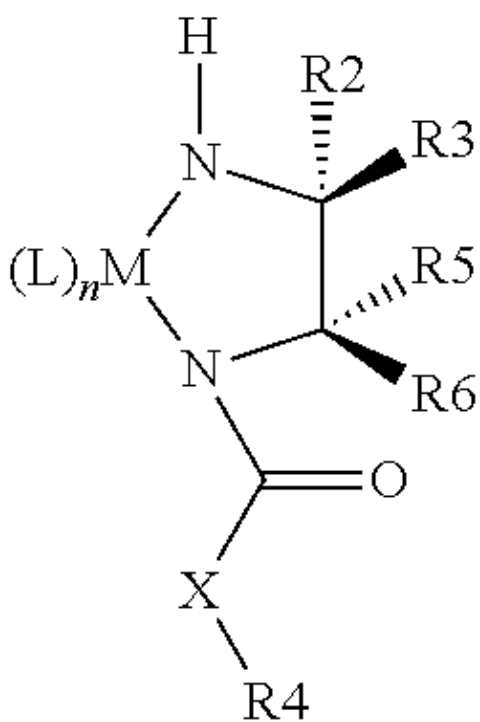
amido-ureate (X = NH) amido-carbamate (X = O)
