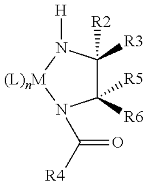
amido-amidate (exocyclic amide)
